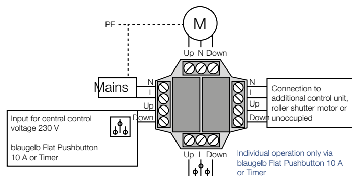
Connection diagram for one roller shutter motor
