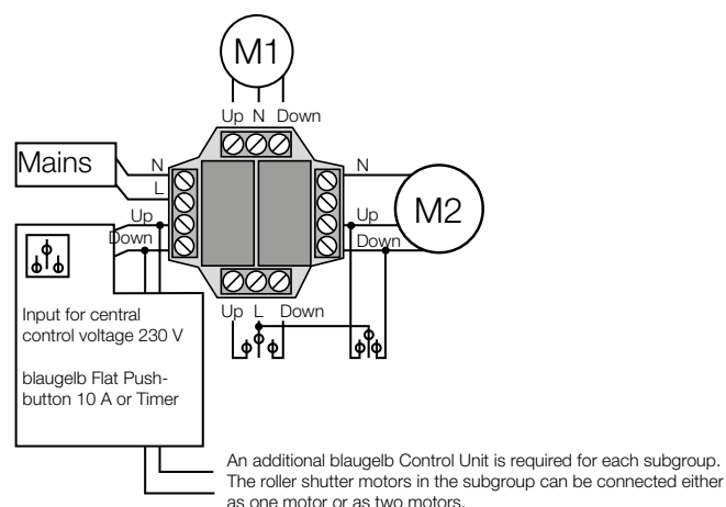
Connection diagram for two roller shutter motors
