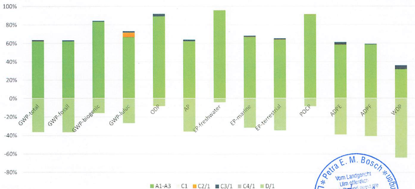
Relative contributions of the various life cycle phases of the blaugelb Insulation Panel MultiPro EPS (100 % material recycling)
